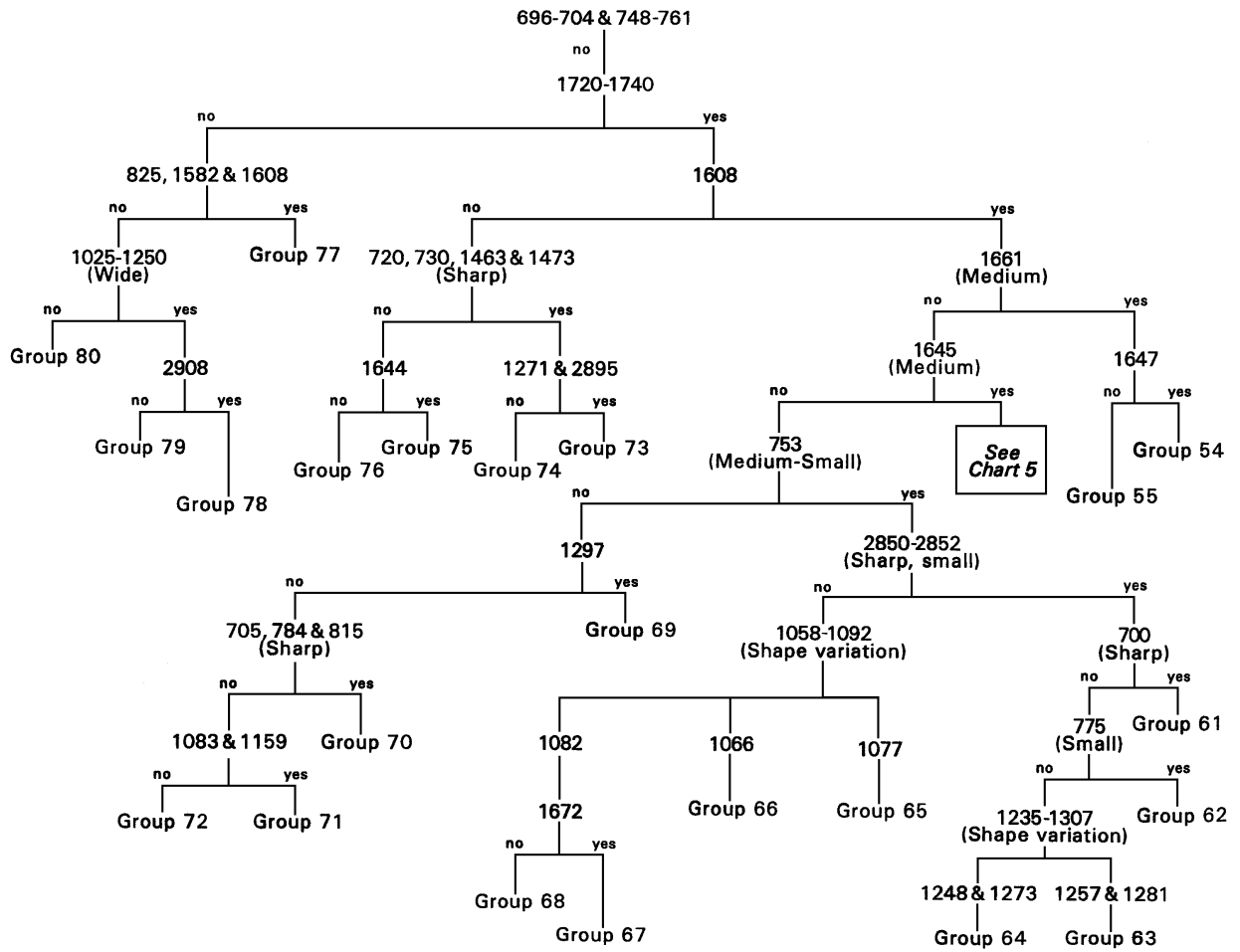
Chart 4. Decision flowchart for copy toner group identification based on R-A IR spectra.
