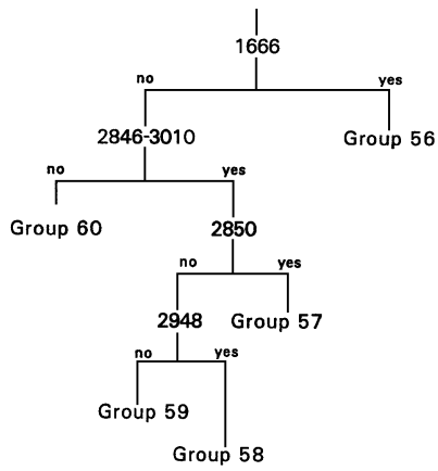
Chart 5. Decision flowchart for copy toner group identification based on R-A IR spectra.
