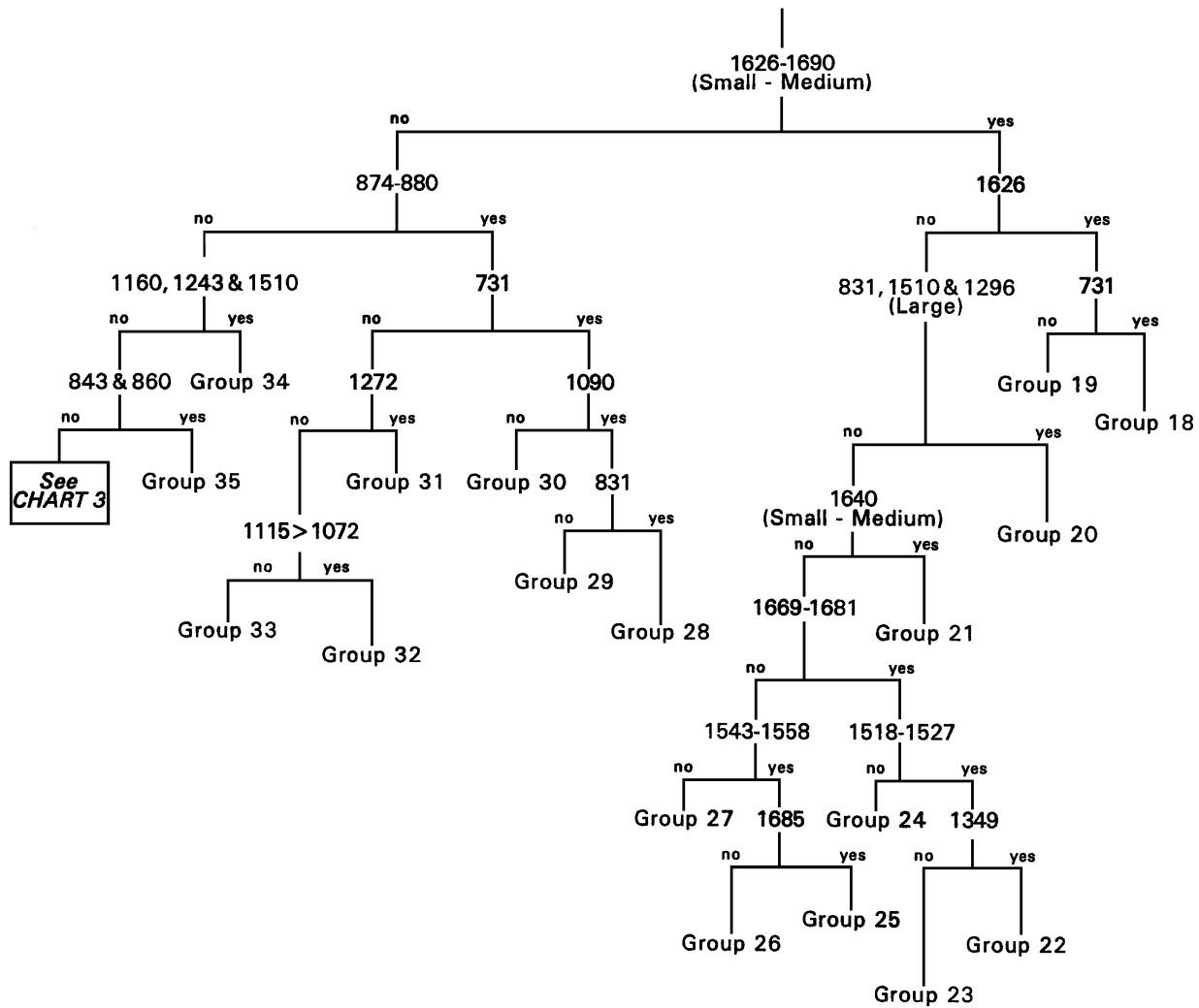
Chart 2. Decision flowchart for copy toner group identification based on R-A IR spectra.
