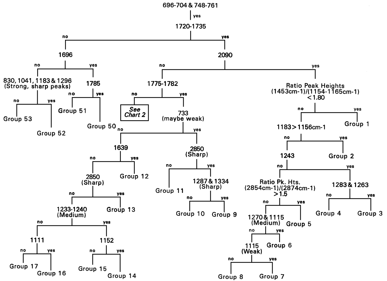
Chart 1. Decision flowchart for copy toner group identification based on R-A IR spectra.
