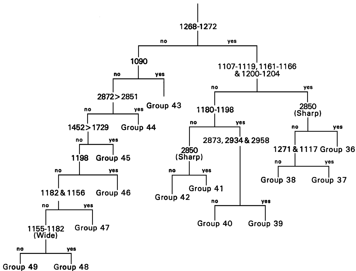
Chart 3. Decision flowchart for copy toner group identification based on R-A IR spectra.
